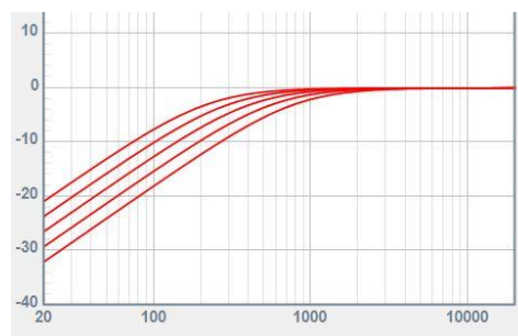
Adjustable HPF
