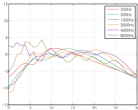
Above: Abscissa: distance (m) ; Column SA250S at 2,55m from ground 0dB is the mean SPL over 5m-20m on axis
